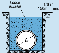
FLAT SUBGRADE CLASS D
