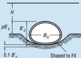
CLASS C
