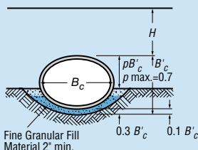
CLASS B
