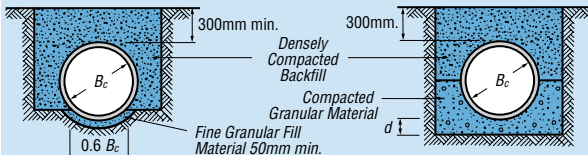
SHAPED SUBGRADE WITH GRANULAR FOUNDATION
