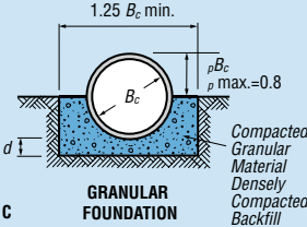
GRANULAR FOUNDATION
