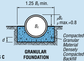
GRANULAR FOUNDATION
