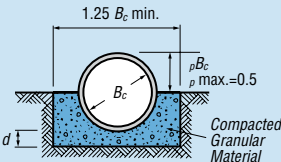
GRANULAR FOUNDATION
