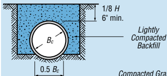
SHAPED SUBGRADE
