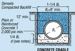
CONCRETE CRADLE
