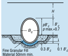
CLASS B
