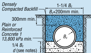
CONCRETE CRADLE
