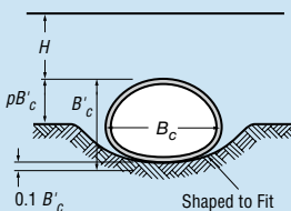
CLASS C
