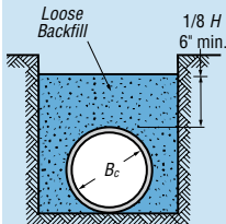
FLAT SUBGRADE CLASS D B_f = 1.1
