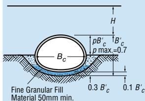
CLASS B
