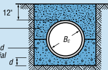
GRANULAR FOUNDATION
