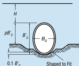
CLASS C
